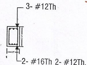
SECTION AT B-B
