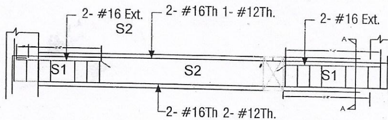
GRID BEAM -DETAILS - A
