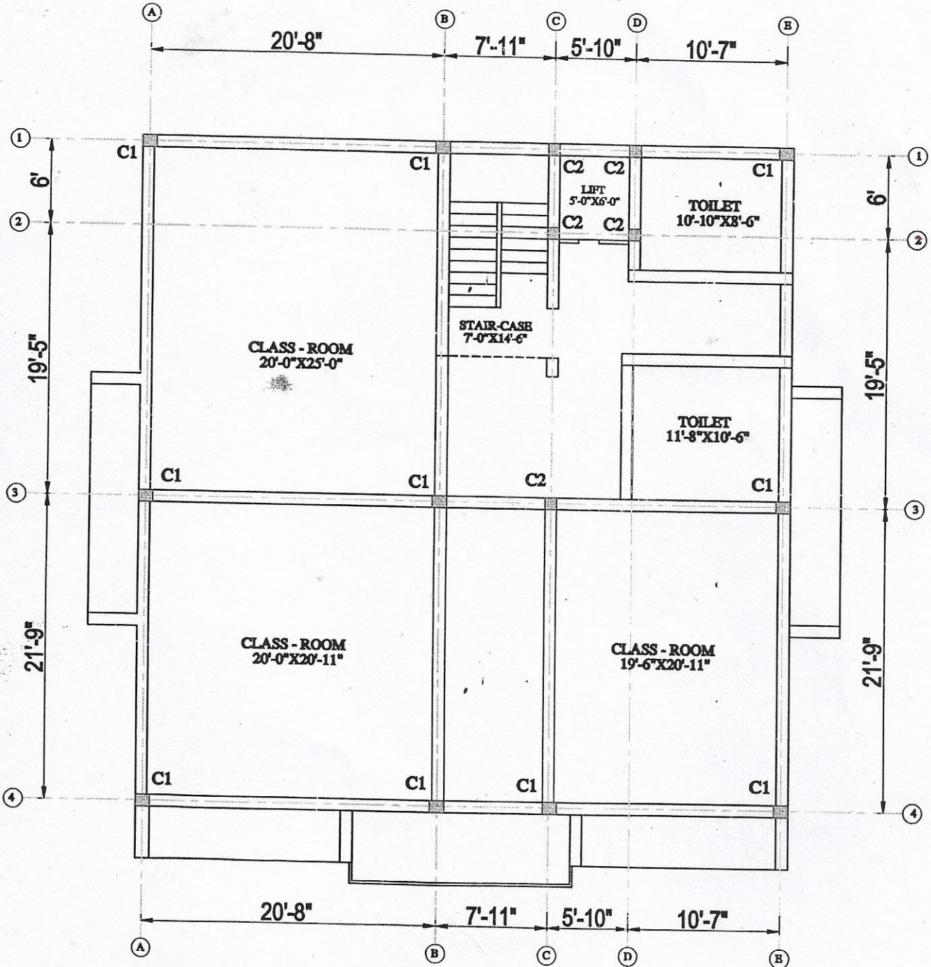
COLUMN LAYOUT- PLAN
