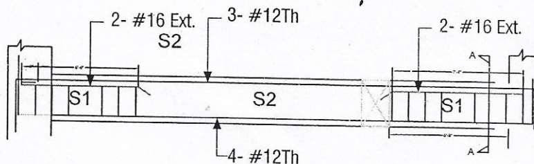
GRID BEAM -DETAILS - C
