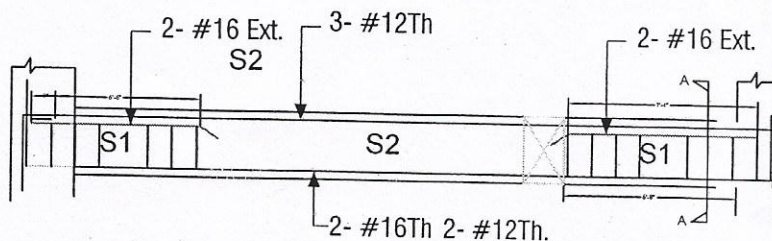
GRID BEAM -DETAILS - B
